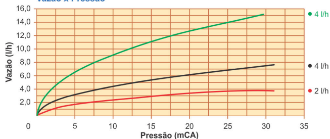
Agri Drip Standard Barb
