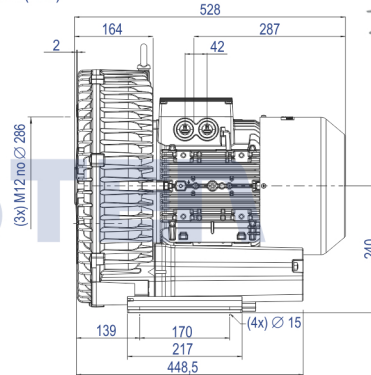
Dimensional (mm)
