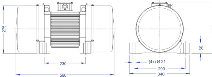
Dimensional (mm)
