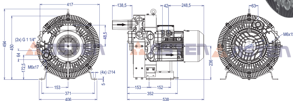
Dimensional (mm)
